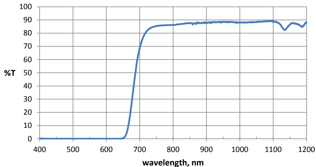
Transmittance spectrum of Luminate 7778 (1.0 mm)
