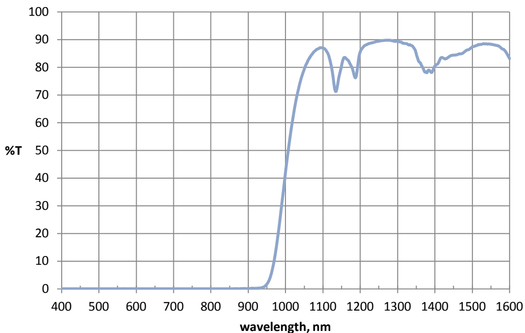
Transmittance spectrum Luminate 7276E (2.84 mm)
