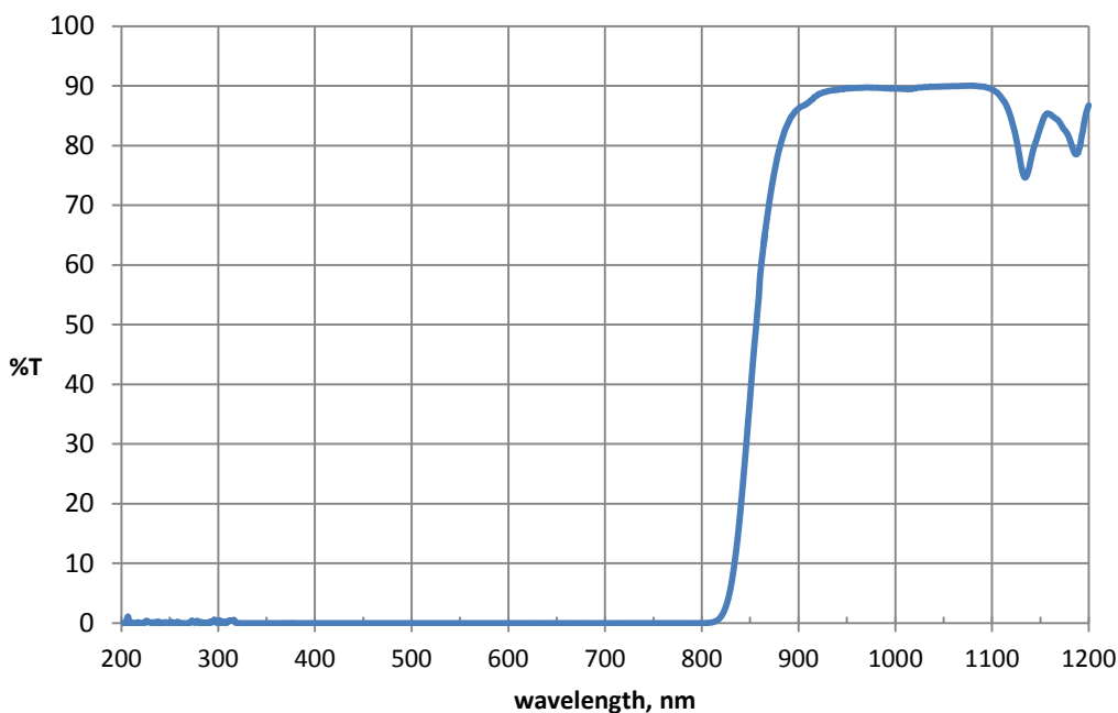
Transmittance spectrum of Epilight 7276A in polycarbonate
