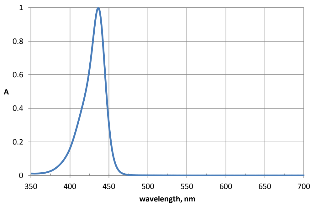
Absorbance spectrum Epilight 5852 in chloroform
