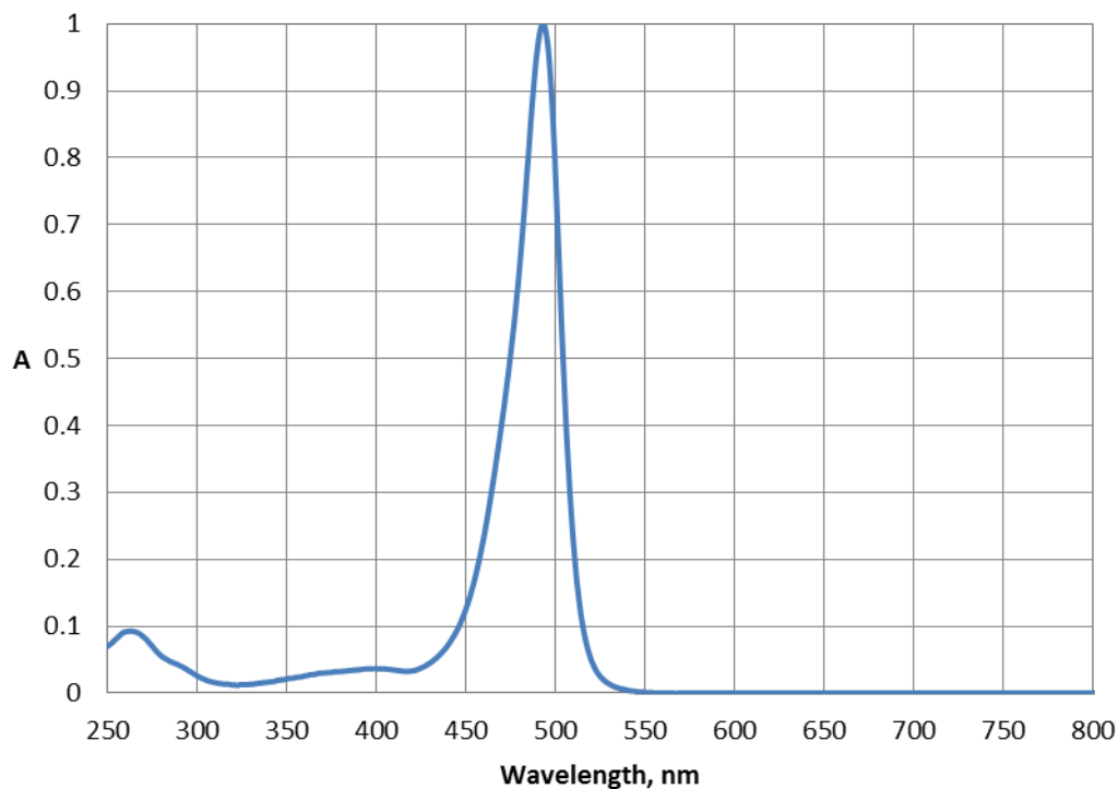
Absorbance spectrum Epolight 5841 in chloroform
